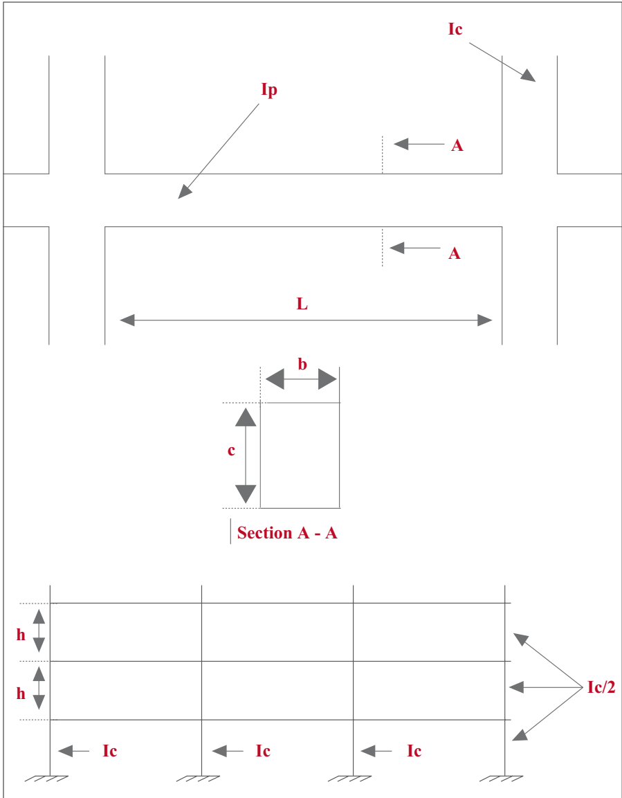
Figure 6.2 : Poutres- poteaux
